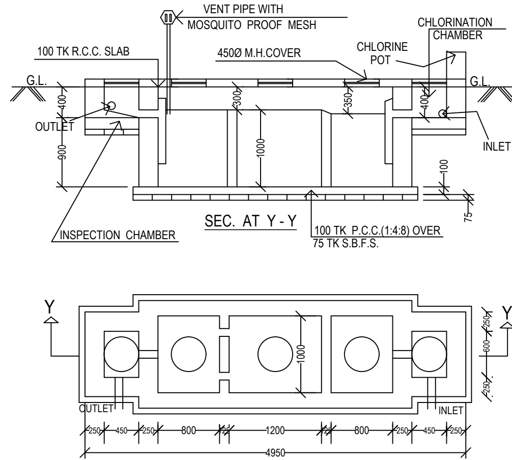
PLAN DETAILS OF SEPTIC TANK SCALE:-1:50 USER-35
